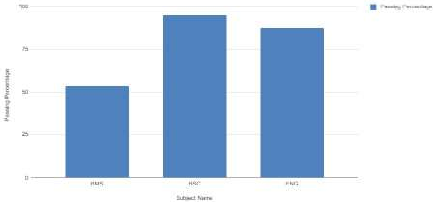
Passing Percentage vs. Subject Name
